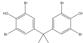
Tetrabromobisphenol A
