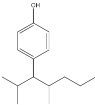
Nonylphenol
